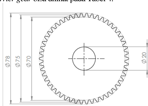
Gambar 4. Hasil desain carrier gear
