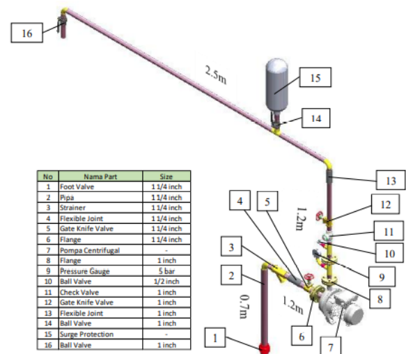
Gambar 2. Desain 3D prototype pipa industri
