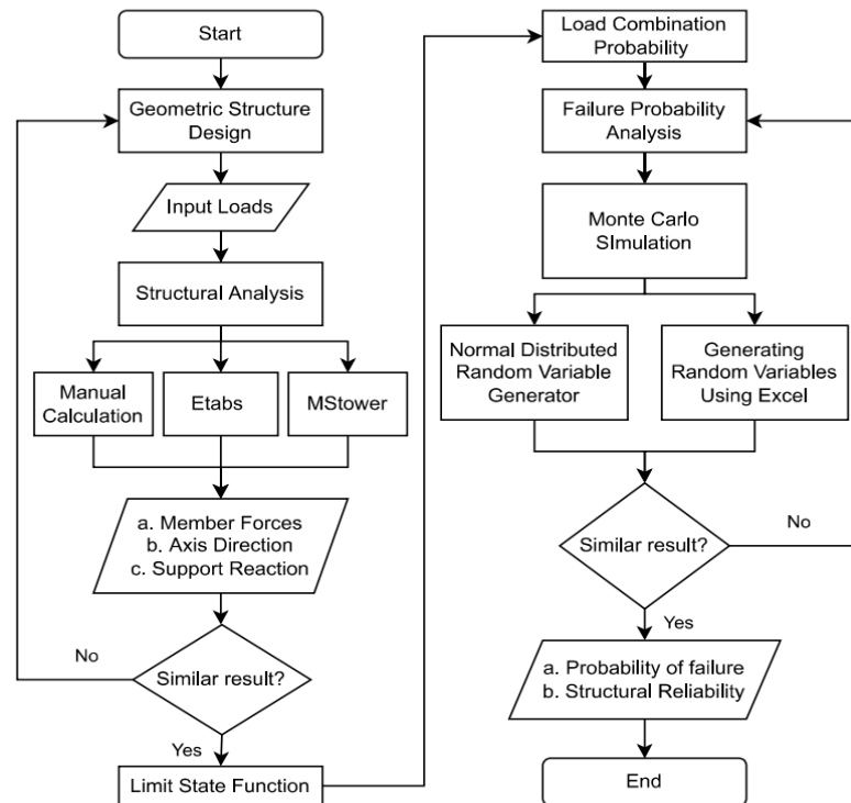
Figure 2. Structural Reliability Analysis Flow Chart
