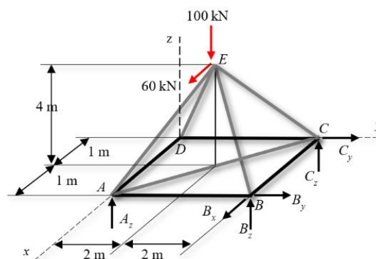
Figure 1. Simple Space Truss Structure (Adapted from Kassimali, 2011)
