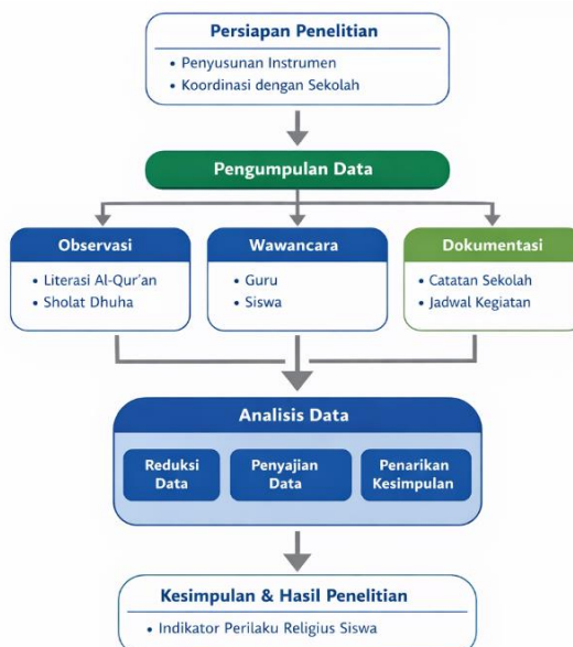
Gambar 1. Alur Penelitian
