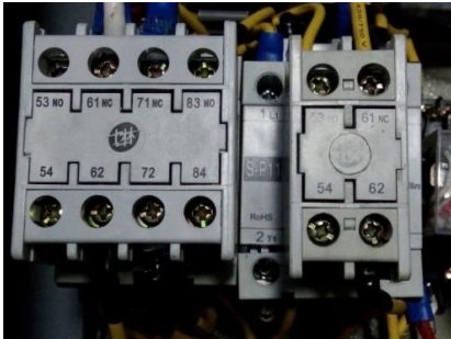
Gambar 16 Magnetic Contactor
