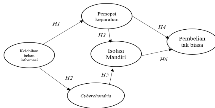
Gambar 1: Model Konseptual
